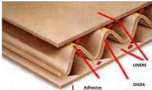
Figure 1. Location of a wave paper in corrugated cardboard.
