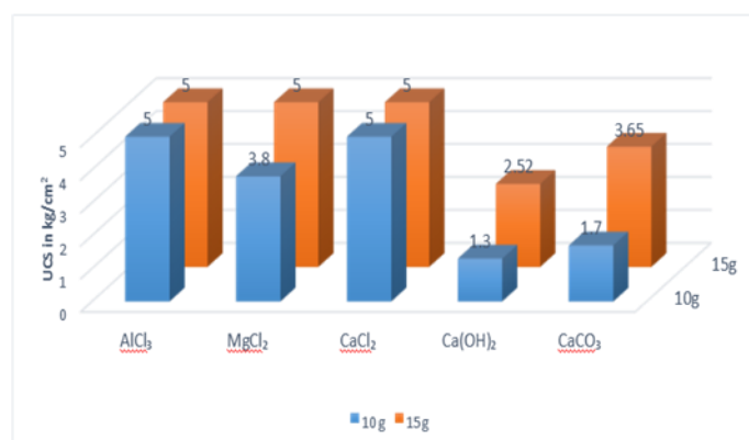
Figure 4. Penetrometer confirmation (in kg/cm 2 ) of the stabilization of 10g and 15g each of the erosive soil using the chemicals
