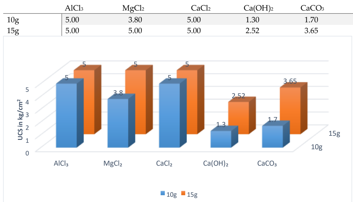
Figure 4. Penetrometer confirmation (in kg/cm 2 ) of the stabilization of 10g and 15g each of the erosive soil using the chemicals DISCUSSION Particle size distribution
